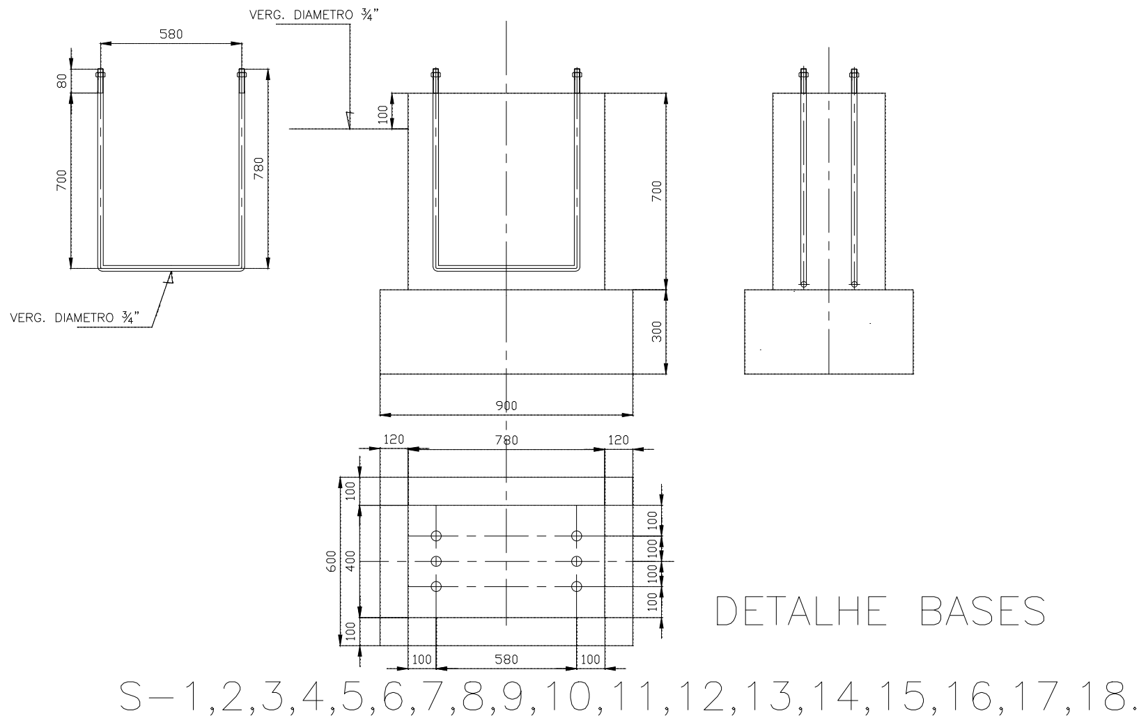
FORMA E FERRAGEM DAS BASES S-1,2,3,4,5,6,7,8,9,10,11,12,13,14, 15,16,17,18.
