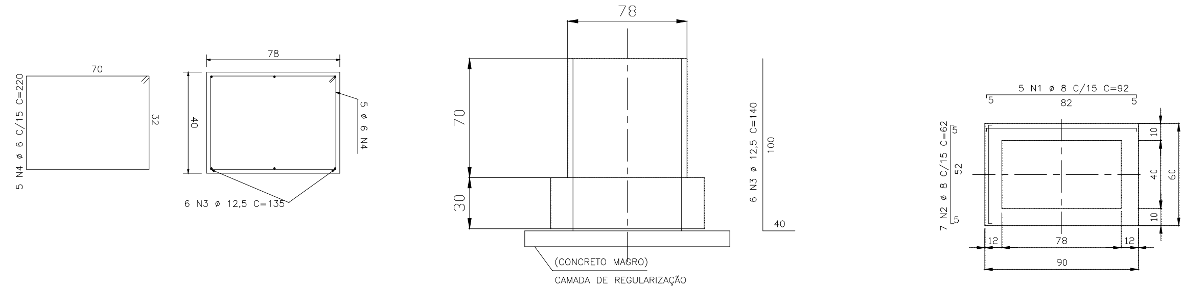
FORMA E FERRAGEM DAS BASES S-1,2,3,4,5,6,7,8,9,10,11,12,13,14, 15,16,17,18.
